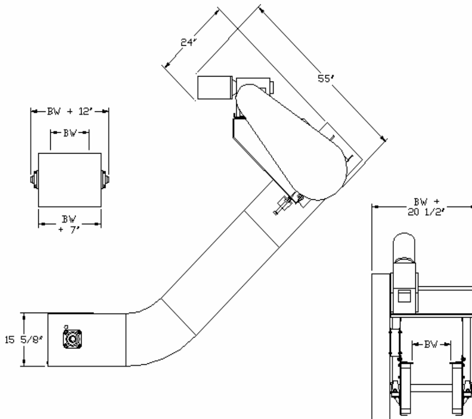
45° TOP MOUNT DRIVE
